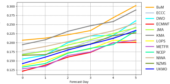
Root mean square error | significant wave height | Gulf of Mexico 20220601 00z to 20220831 00z | waveapi lw wave prod 00z mean_fair
