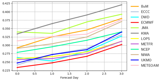
Scatter index | significant wave height | Mediterranean 20220601 00z to 20220831 00z | waveapi lw wave prod 00z mean_fair
