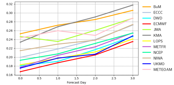
Root mean square error | significant wave height | Mediterranean 20220601 00z to 20220831 00z | waveapi lw wave prod 00z mean_fair
