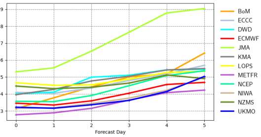
Root mean square error | significant wave height | South Southwestern Austr 20220601 00z to 20220831 00z | waveapi lw wave prod 00z mean_fair
