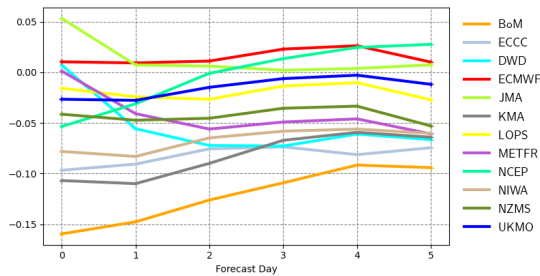
Mean error | significant wave height | Gulf of Mexico 20220601 00z to 20220831 00z | waveapi lw wave prod 00z mean_fair
