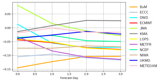
Mean error | significant wave height | Mediterranean 20220601 00z to 20220831 00z | waveapi lw wave prod 00z mean_fair
