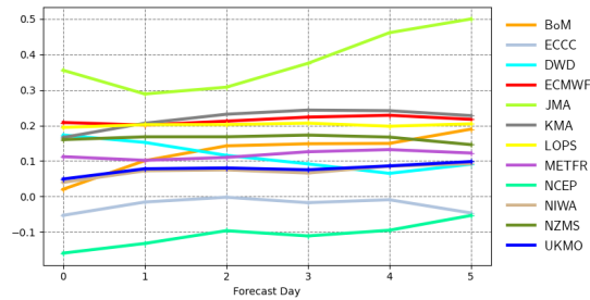
Mean error | significant wave height | South Southwestern Australia 20220601 00z to 20220831 00z | waveapi lw wave prod 00z mean_fair
