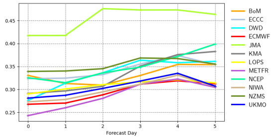
Root mean square error | significant wave height | South Southwestern Aust 20221201 00z to 20230228 00z | waveapi lw wave prod 00z mean_fair
