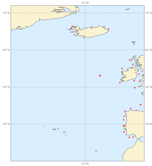
Buoys observations - from 20221201 to 20230228 - (swh)
