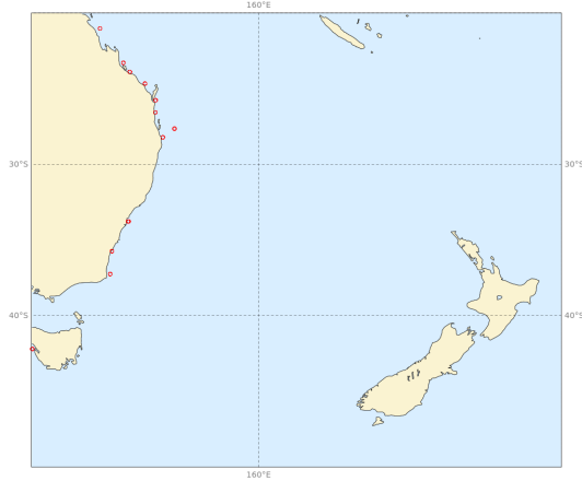
Buoys observations - from 20221201 to 20230228 - (swh)
