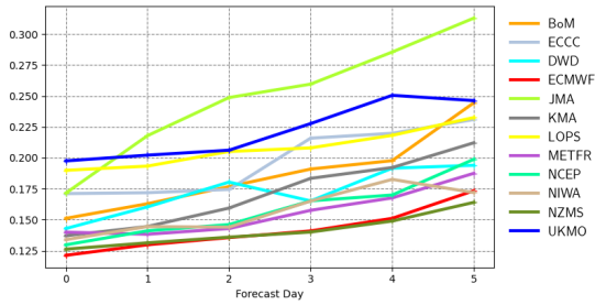
Scatter index | significant wave height | Eastern Australia and New Zealand 20230901 00z to 20231130 00z | waveapi lw wave prod 00z mean_fair
