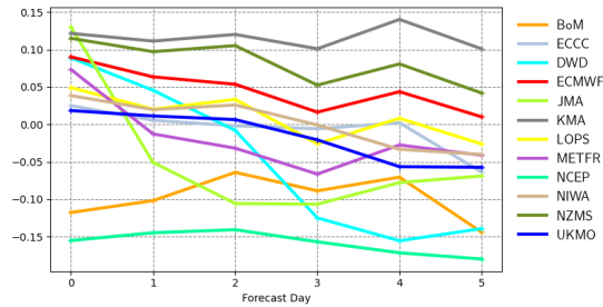
Mean error | significant wave height | South Southwestern Australia 20230901 00z to 20231130 00z | waveapi lw wave prod 00z mean_fair
