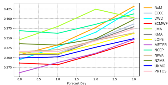
Root mean square error | significant wave height | SW Europe 20230901 00z to 20231130 00z | waveapi lw wave prod 00z mean_fair
