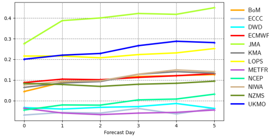
Mean error | significant wave height | Eastern Australia and New Zealand 20230901 00z to 20231130 00z | waveapi lw wave prod 00z mean_fair
