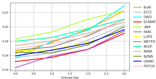
Scatter index | significant wave height | SW Europe 20230901 00z to 20231130 00z | waveapi lw wave prod 00z mean_fair
