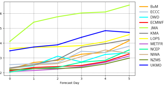
Root mean square error | significant wave height | Eastern Australia and New Zealand 20230901 00z to 20231130 00z | waveapi lw wave prod 00z mean_fair
