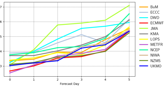
Root mean square error | significant wave height | South Southwestern Austr 20230901 00z to 20231130 00z | waveapi lw wave prod 00z mean_fair
