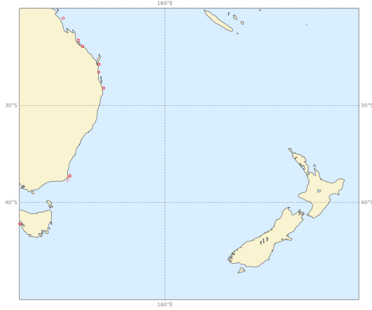
Scatter index | significant wave height | Eastern Australia and New Zealand 20230901 00z to 20231130 00z | waveapi lw wave prod 00z mean_fair
