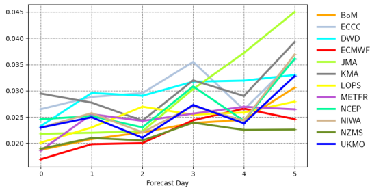
Scatter index | significant wave height | South Southwestern Australia 20230901 00z to 20231130 00z | waveapi lw wave prod 00z mean_fair
