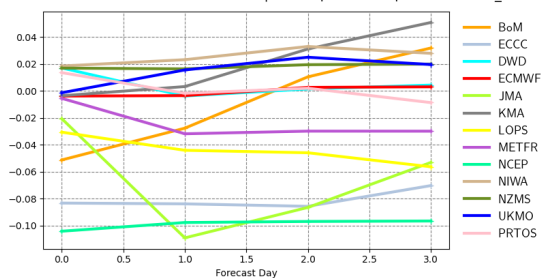
Mean error | significant wave height | SW Europe 20230901 00z to 20231130 00z | waveapi lw wave prod 00z mean_fair
