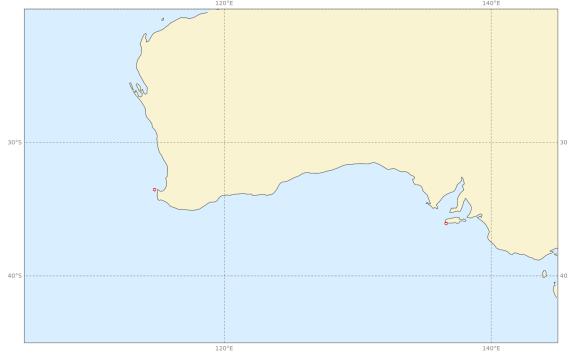
Scatter index | significant wave height | South Southwestern Australia 20230901 00z to 20231130 00z | waveapi lw wave prod 00z mean_fair
