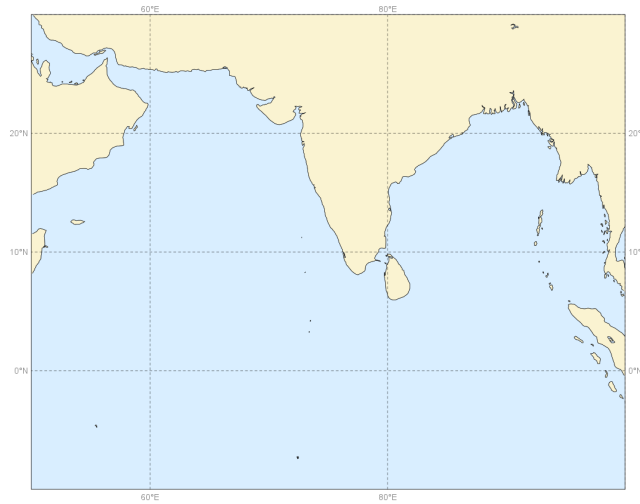
Buoys observations - from 20181201 to 20190228 - (pp1d)
