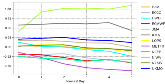
Mean error | pp1d | Eastern Australia and New Zealand 20211201 00z to 20220228 00z | waveapi lw wave prod 00z mean_fair
