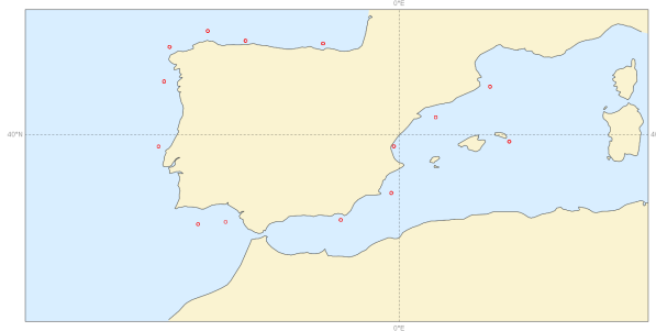
Scatter index | pp1d | SW Europe 20211201 00z to 20220228 00z | waveapi lw wave prod 00z mean_fair
