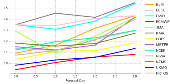
Mean error | pp1d | SW Europe 20211201 00z to 20220228 00z | waveapi lw wave prod 00z mean_fair
