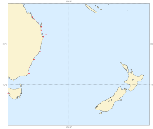
Scatter index | pp1d | Eastern Australia and New Zealand 20211201 00z to 20220228 00z | waveapi lw wave prod 00z mean_fair
