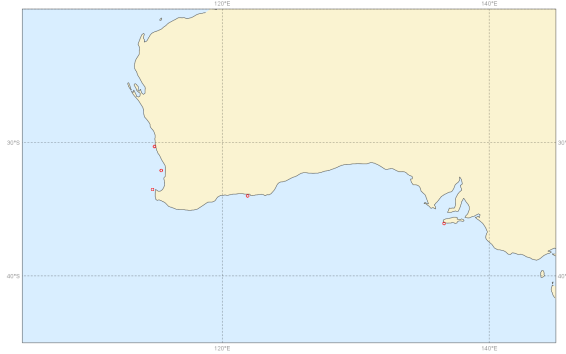
Buoys observations - from 20211201 to 20220228 - (pp1d)
