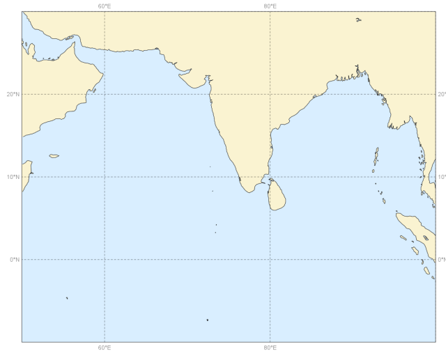
Buoys observations - from 20211201 to 20220228 - (pp1d)
