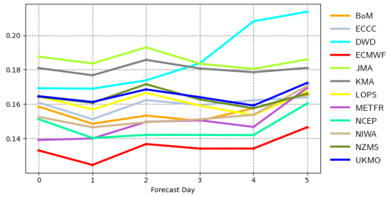
Scatter index | pp1d | Eastern Australia and New Zealand 20211201 00z to 20220228 00z | waveapi lw wave prod 00z mean_fair
