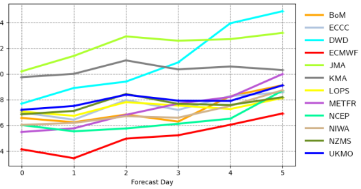
Root mean square error | pp1d | Eastern Australia and New Zealand 20211201 00z to 20220228 00z | waveapi lw wave prod 00z mean_fair
