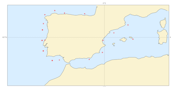
Scatter index | pp1d | SW Europe 20231201 00z to 20240229 00z | waveapi lw wave prod 00z mean_fair
