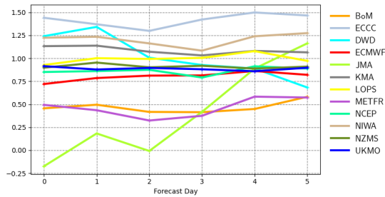
Mean error | pp1d | South Southwestern Australia 20231201 00z to 20240229 00z | waveapi lw wave prod 00z mean_fair
