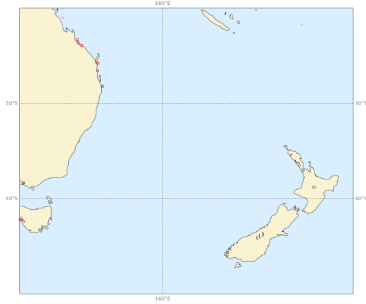
Buoys observations - from 20231201 to 20240229 - (pp1d)
