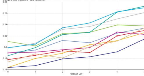
pp1d Scatter index Europe (lat: 35.0 to 75.0, lon: -12.5 to 42.5) Date: 20190901 00UTC to 20191130 00UTC Average for every grid 00UTC. Mean method for
