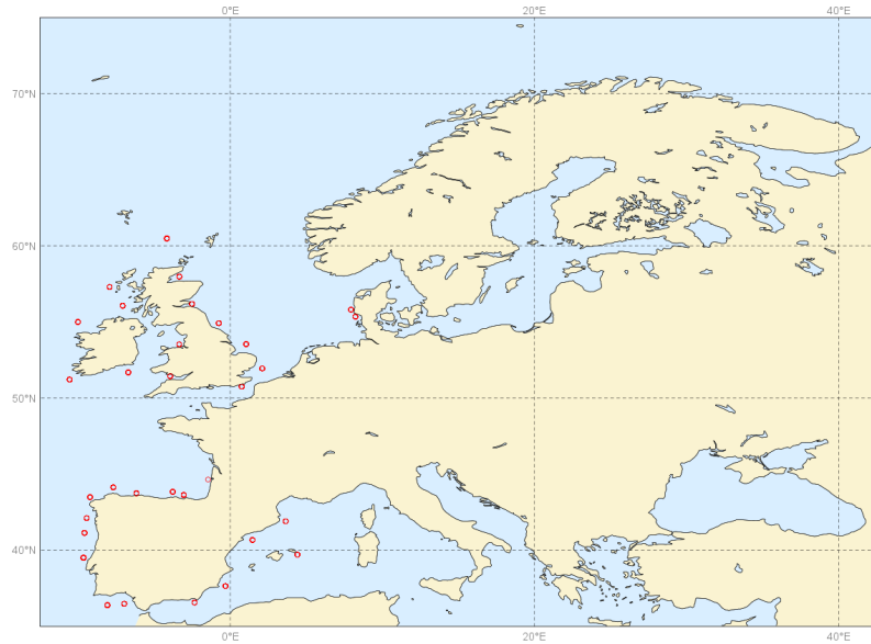
pp1d Scatter index Europe (lat: 35.0 to 75.0, lon: -12.5 to 42.5) Date: 20190901 00UTC to 20191130 00UTC Average for every grid 00UTC. Mean method for
