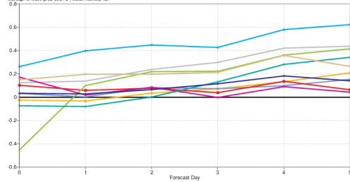
pp1d Mean error Europe (lat: 35.0 to 75.0, lon: -12.5 to 42.5) Date: 20190901 00UTC to 20191130 00UTC Average for every grid 00UTC. Mean method for
