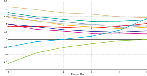
pp1d Mean error North East Pacific (lat 30 to 62, lon -180 to -115) Date: 20190901 00UTC to 20191130 00UTC averaged by wave period (0UTC), Mean method (lat)
