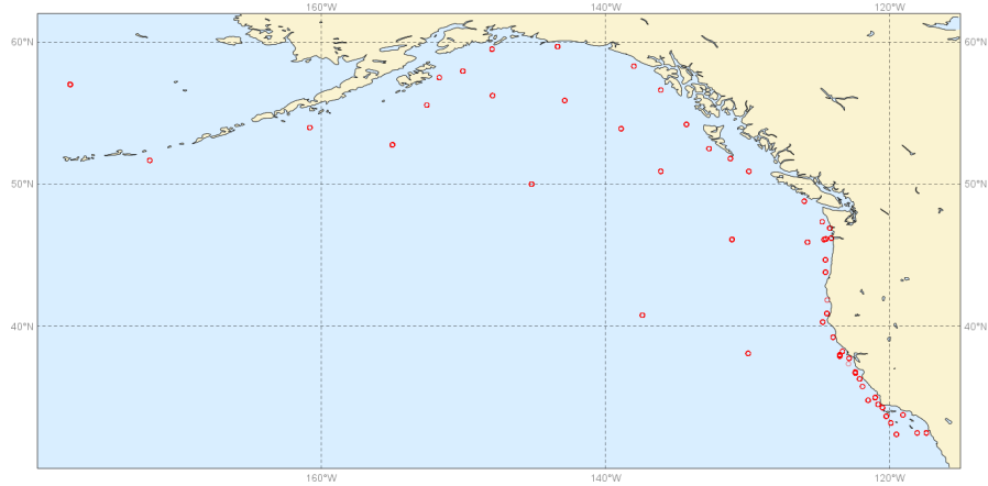
pp1d Scatter index North East Pacific (lat 30 to 62, lon -180 to -115) Date: 20190901 00UTC to 20191130 00UTC averaged by wave period (0UTC), Mean method (lat)
