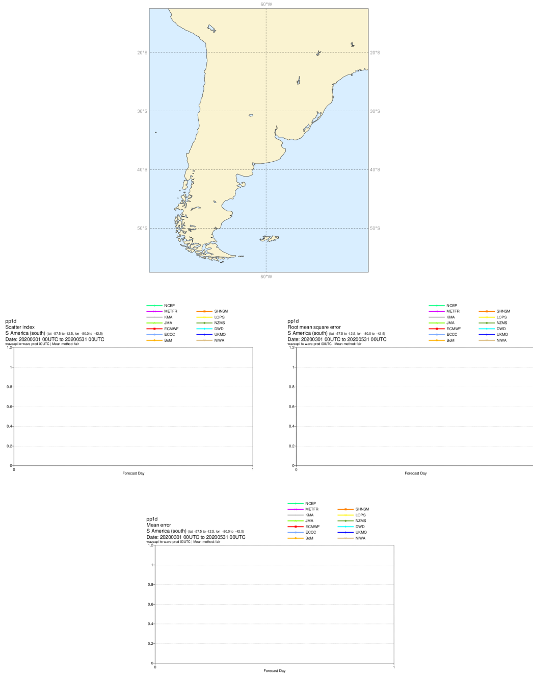
South of South America. Top panel: observation distribution. Middle left panel: Forecast scatter index (standard deviation of the difference normalised by the mean of the observations). Middle right panel: Forecast root mean square error (RMSE). Bottom panel: forecast mean error (bias).
