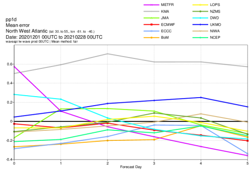
North West Atlantic. Top panel: observation distribution. Middle left panel: Forecast scatter index (standard deviation of the difference normalised by the mean of the observations). Middle right panel: Forecast root mean square error (RMSE). Bottom panel: forecast mean error (bias).
