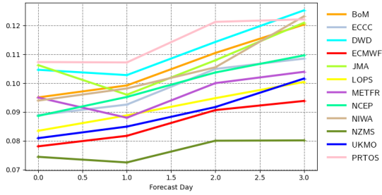
Mean error | pp1d | SW Europe 20211201 00z to 20220228 12z | waveapi lw wave prod mean_fair
