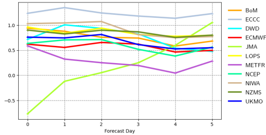
Mean error | pp1d | South Southwestern Australia 20211201 00z to 20220228 12z | waveapi lw wave prod mean_fair
