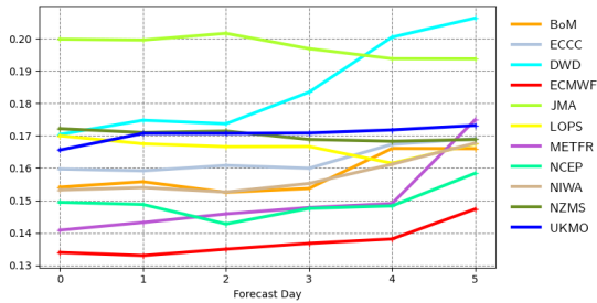
Scatter index | pp1d | Eastern Australia and New Zealand 20211201 00z to 20220228 12z | waveapi lw wave prod mean_fair
