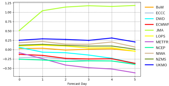
Mean error | pp1d | Eastern Australia and New Zealand 20211201 00z to 20220228 12z | waveapi lw wave prod mean_fair
