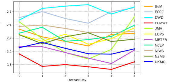
Root mean square error | pp1d | South Southwestern Australia 20211201 00z to 20220228 12z | waveapi lw wave prod mean_fair
