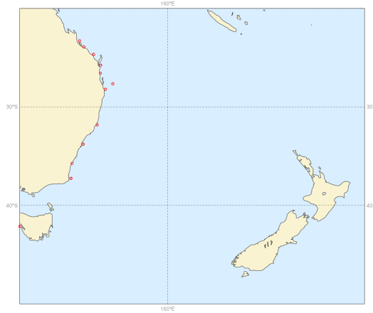
Scatter index | pp1d | Eastern Australia and New Zealand 20211201 00z to 20220228 12z | waveapi lw wave prod mean_fair
