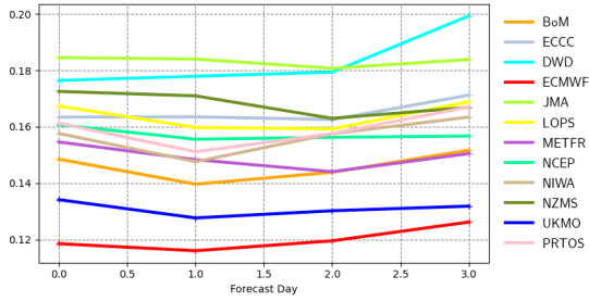
Mean error | pp1d | SW Europe 20220601 00z to 20220831 12z | waveapi lw wave prod mean_fair
