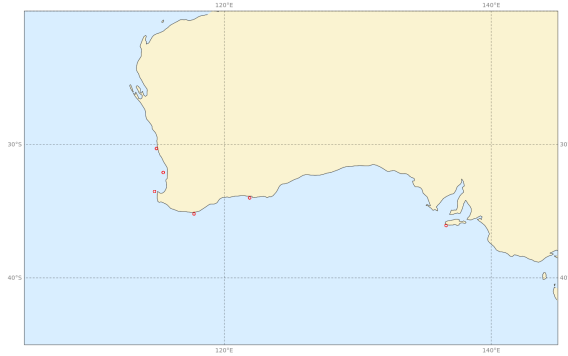
Scatter index | pp1d | South Southwestern Australia 20220601 00z to 20220831 12z | waveapi lw wave prod mean_fair
