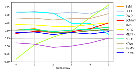
Mean error | pp1d | South Southwestern Australia 20220601 00z to 20220831 12z | waveapi lw wave prod mean_fair
