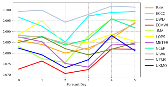
Scatter index | pp1d | South Southwestern Australia 20220601 00z to 20220831 12z | waveapi lw wave prod mean_fair
