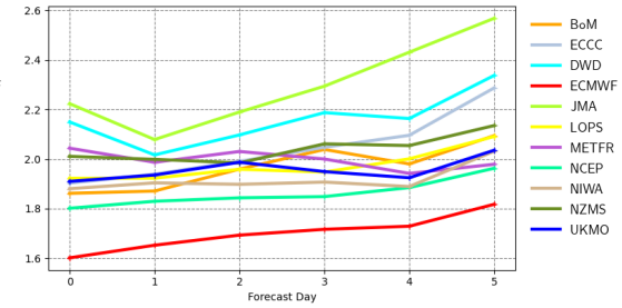
Root mean square error | pp1d | Eastern Australia and New Zealand 20220601 00z to 20220831 12z | waveapi lw wave prod mean_fair
