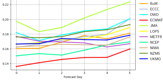
Mean error | pp1d | Eastern Australia and New Zealand 20220601 00z to 20220831 12z | waveapi lw wave prod mean_fair
