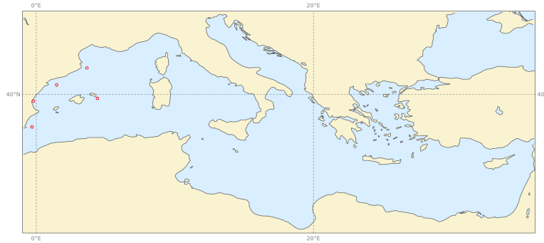
Buoys observations - from 20220601 to 20220831 - (pp1d)
