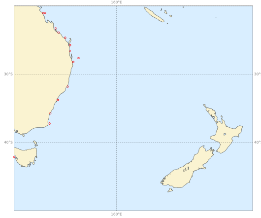
Scatter index | pp1d | Eastern Australia and New Zealand 20220601 00z to 20220831 12z | waveapi lw wave prod mean_fair
