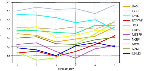
Root mean square error | pp1d | South Southwestern Australia 20220601 00z to 20220831 12z | waveapi lw wave prod mean_fair
