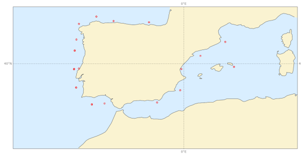
Scatter index | pp1d | SW Europe 20220601 00z to 20220831 12z | waveapi lw wave prod mean_fair
