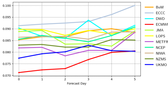
Scatter index | pp1d | South Southwestern Australia 20220301 00z to 20220530 12z | waveapi lw wave prod mean_fair
