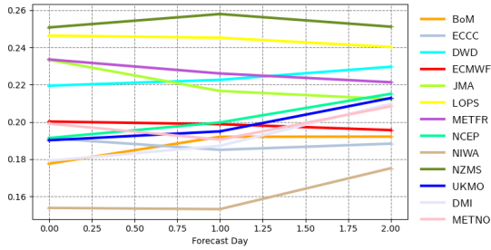
Scatter index | pp1d | North Sea 20220301 00z to 20220530 12z | waveapi lw wave prod mean_fair
