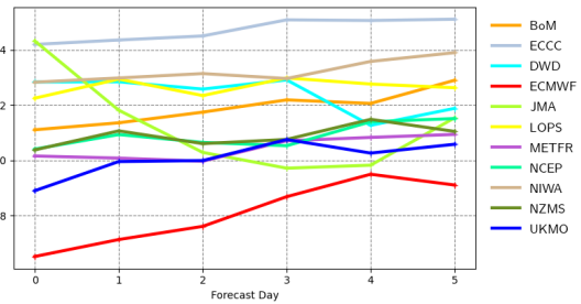
Root mean square error | pp1d | South Southwestern Australia 20220301 00z to 20220530 12z | waveapi lw wave prod mean_fair
