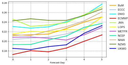
Mean error | pp1d | Europe 20220301 00z to 20220530 12z | waveapi lw wave prod mean_fair
