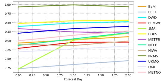
Mean error | pp1d | North Sea 20220301 00z to 20220530 12z | waveapi lw wave prod mean_fair
