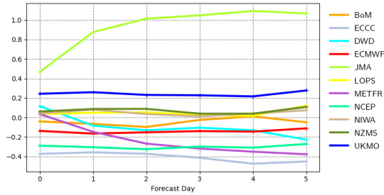
Mean error | pp1d | Eastern Australia and New Zealand 20220301 00z to 20220530 12z | waveapi lw wave prod mean_fair
