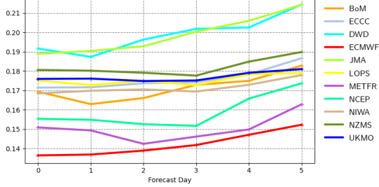
Mean error | pp1d | Eastern Australia and New Zealand 20220301 00z to 20220530 12z | waveapi lw wave prod mean_fair
