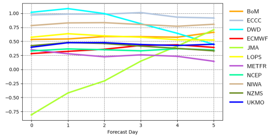
Mean error | pp1d | South Southwestern Australia 20220301 00z to 20220530 12z | waveapi lw wave prod mean_fair
