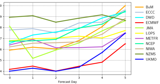
Root mean square error | pp1d | North East Atlantic 20230901 00z to 20231130 12z | waveapi lw wave prod mean_fair
