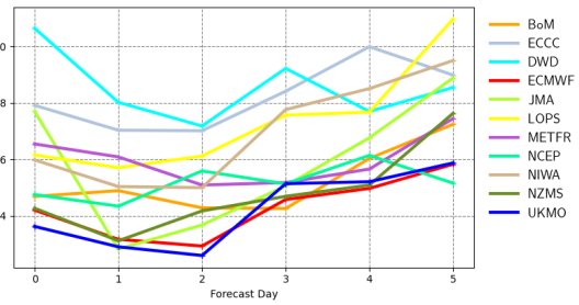
Root mean square error | pp1d | South Southwestern Australia 20230901 00z to 20231130 12z | waveapi lw wave prod mean_fair
