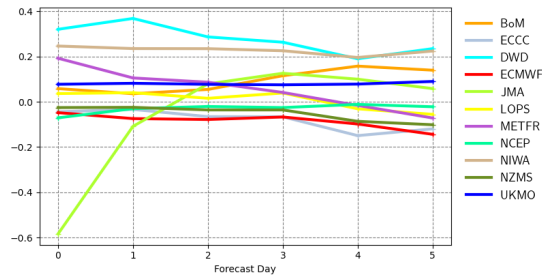
Mean error | pp1d | Europe 20230901 00z to 20231130 12z | waveapi lw wave prod mean_fair
