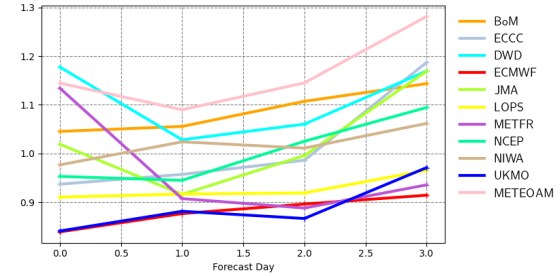
Root mean square error | pp1d | Mediterranean 20230901 00z to 20231130 12z | waveapi lw wave prod mean_fair
