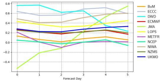
Mean error | pp1d | South Southwestern Australia 20230901 00z to 20231130 12z | waveapi lw wave prod mean_fair
