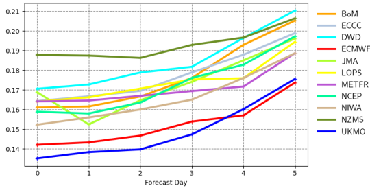
Scatter index | pp1d | Europe 20230901 00z to 20231130 12z | waveapi lw wave prod mean_fair
