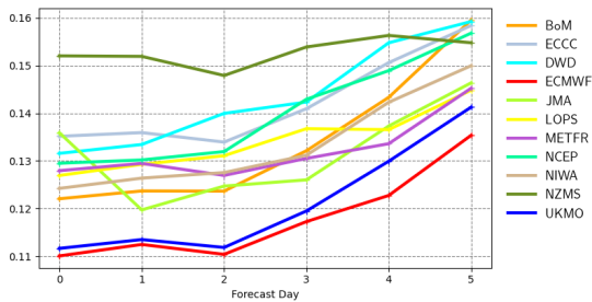
Scatter index | pp1d | North East Atlantic 20230901 00z to 20231130 12z | waveapi lw wave prod mean_fair
