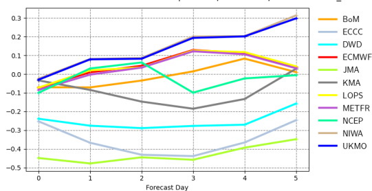
Mean error | 10m wind speed | Hawaii 20221201 00z to 20230228 00z | waveapi lw wave prod 00z mean_fair
