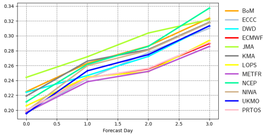
Scatter index | 10m wind speed | SW Europe 20221201 00z to 20230228 00z | waveapi lw wave prod 00z mean_fair
