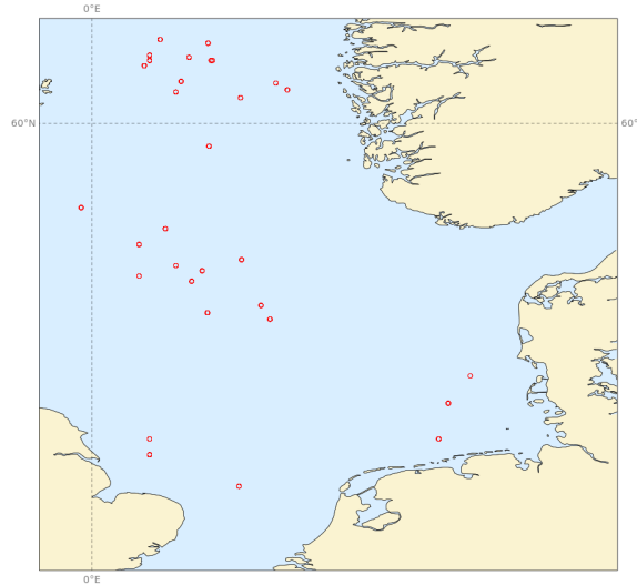
Buoys observations - from 20221201 to 20230228 - (10ff)
