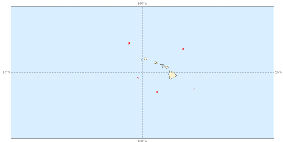
Scatter index | 10m wind speed | Hawaii 20221201 00z to 20230228 00z | waveapi lw wave prod 00z mean_fair
