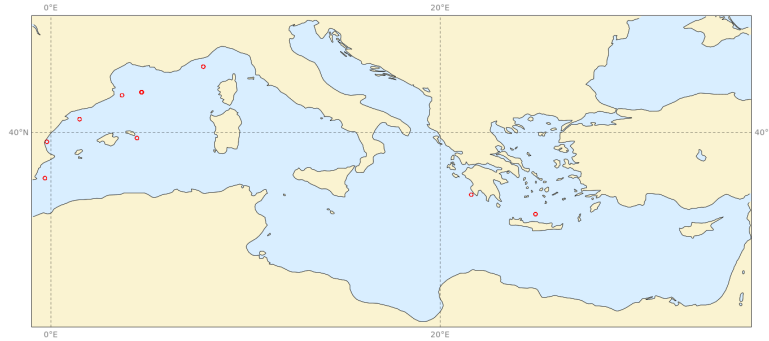
Buoys observations - from 20221201 to 20230228 - (10ff)
