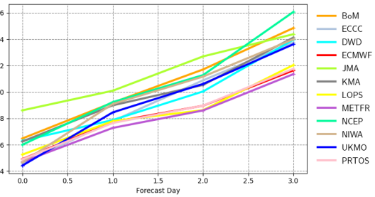
Root mean square error | 10m wind speed | SW Europe 20221201 00z to 20230228 00z | waveapi lw wave prod 00z mean_fair
