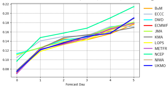
Scatter index | 10m wind speed | Hawaii 20221201 00z to 20230228 00z | waveapi lw wave prod 00z mean_fair
