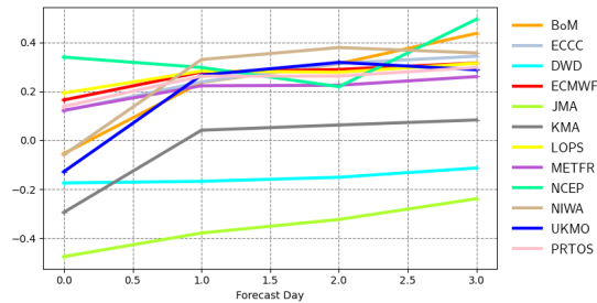
Mean error | 10m wind speed | SW Europe 20221201 00z to 20230228 00z | waveapi lw wave prod 00z mean_fair
