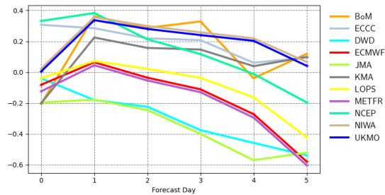
Mean error | 10m wind speed | Europe 20231201 00z to 20240229 00z | waveapi lw wave prod 00z mean_fair
