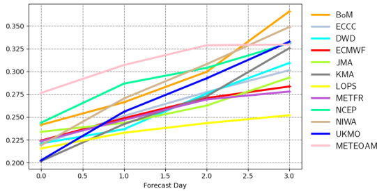
Scatter index | 10m wind speed | Mediterranean 20231201 00z to 20240229 00z | waveapi lw wave prod 00z mean_fair
