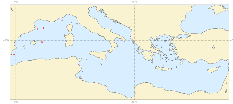
Scatter index | 10m wind speed | Mediterranean 20231201 00z to 20240229 00z | waveapi lw wave prod 00z mean_fair
