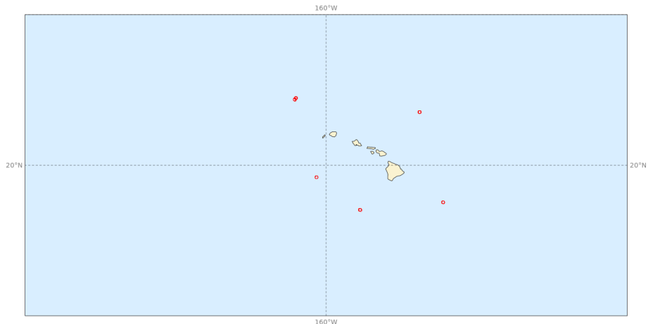
Buoys observations - from 20231201 to 20240229 - (10ff)
