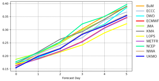
Scatter index | 10m wind speed | Europe 20231201 00z to 20240229 00z | waveapi lw wave prod 00z mean_fair
