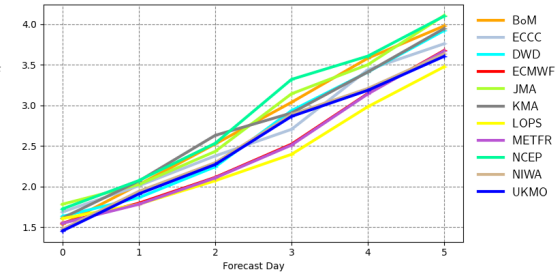
Root mean square error | 10m wind speed | Europe 20231201 00z to 20240229 00z | waveapi lw wave prod 00z mean_fair
