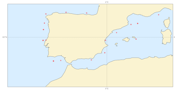
Scatter index | 10m wind speed | SW Europe 20231201 00z to 20240229 00z | waveapi lw wave prod 00z mean_fair
