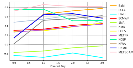
Mean error | 10m wind speed | Mediterranean 20231201 00z to 20240229 00z | waveapi lw wave prod 00z mean_fair
