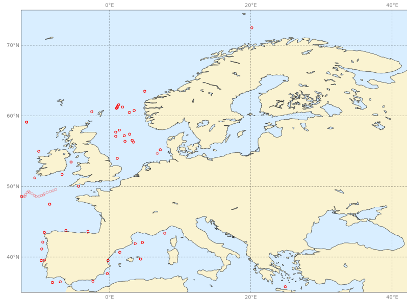
Scatter index | 10m wind speed | Europe 20231201 00z to 20240229 00z | waveapi lw wave prod 00z mean_fair
