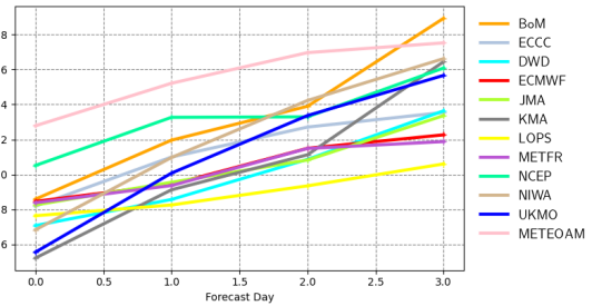
Root mean square error | 10m wind speed | Mediterranean 20231201 00z to 20240229 00z | waveapi lw wave prod 00z mean_fair
