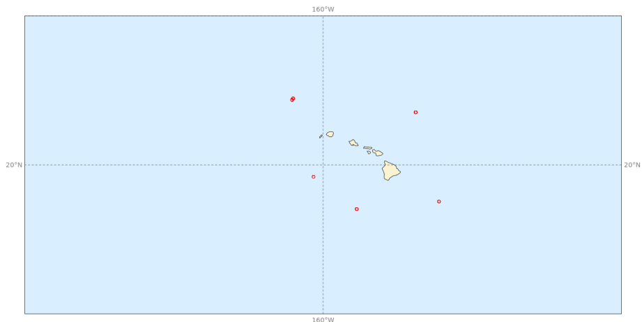
Buoys observations - from 20230901 to 20231130 - (10ff)
