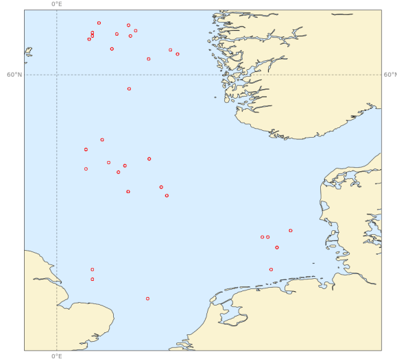
Buoys observations - from 20230901 to 20231130 - (10ff)
