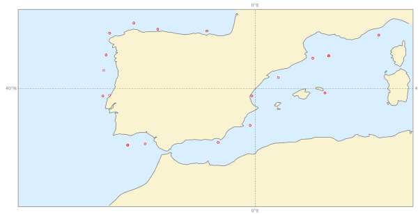
Scatter index | 10m wind speed | SW Europe 20230901 00z to 20231130 00z | waveapi lw wave prod 00z mean_fair
