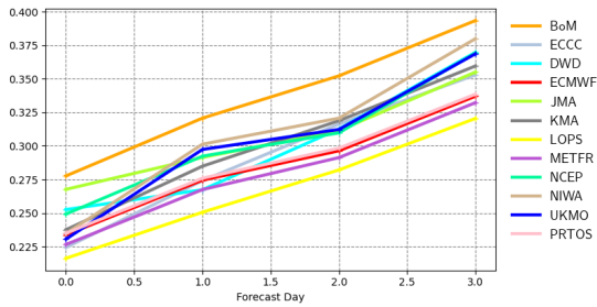
Mean error | 10m wind speed | SW Europe 20230901 00z to 20231130 00z | waveapi lw wave prod 00z mean_fair
