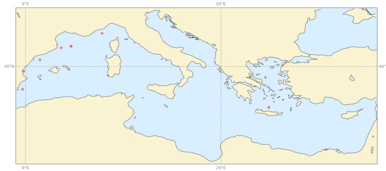
Buoys observations - from 20230901 to 20231130 - (10ff)
