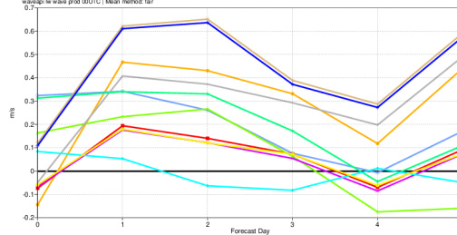
10m wind speed Mean error Europe (lat: 35.0 to 75.0, lon: -12.5 to 42.5) Date: 20210901 00UTC to 20211130 00UTC Average for every grid (0UTC). Mean method for
