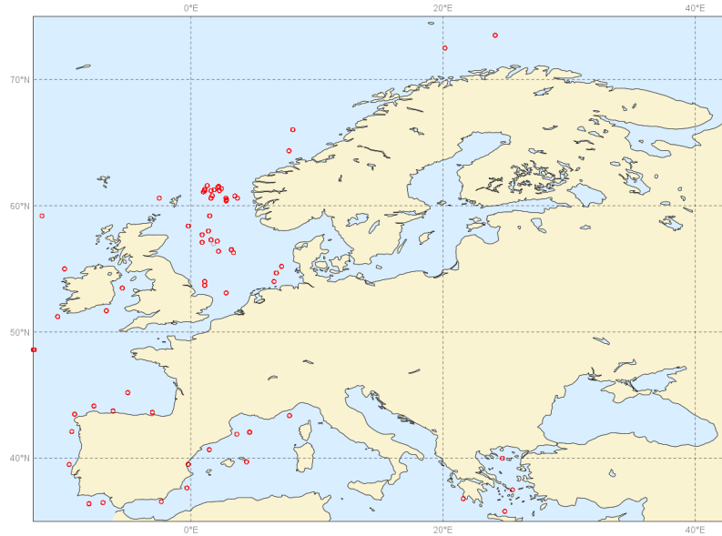
10m wind speed Scatter index Europe (lat: 35.0 to 75.0, lon: -12.5 to 42.5) Date: 20210901 00UTC to 20211130 00UTC Average for every grid (0UTC). Mean method for
