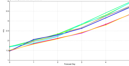
10m wind speed Root mean square error Europe (lat: 35.0 to 75.0, lon: -12.5 to 42.5) Date: 20210901 00UTC to 20211130 00UTC Average for every grid (0UTC). Mean method for
