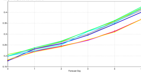
10m wind speed Scatter index Europe (lat: 35.0 to 75.0, lon: -12.5 to 42.5) Date: 20210901 00UTC to 20211130 00UTC Average for every grid (0UTC). Mean method for
