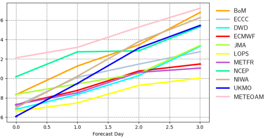
Root mean square error | 10m wind speed | Mediterranean 20231201 00z to 20240229 12z | waveapi lw wave prod mean_fair
