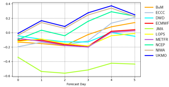
Mean error | 10m wind speed | Gulf of Mexico 20231201 00z to 20240229 12z | waveapi lw wave prod mean_fair
