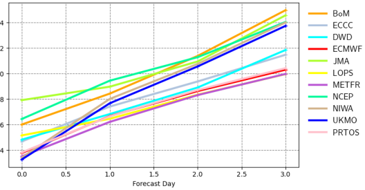
Root mean square error | 10m wind speed | SW Europe 20231201 00z to 20240229 12z | waveapi lw wave prod mean_fair
