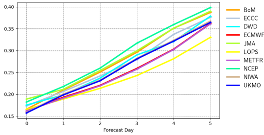
Scatter index | 10m wind speed | Europe 20231201 00z to 20240229 12z | waveapi lw wave prod mean_fair
