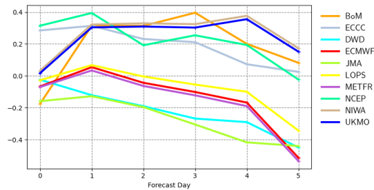
Mean error | 10m wind speed | Europe 20231201 00z to 20240229 12z | waveapi lw wave prod mean_fair
