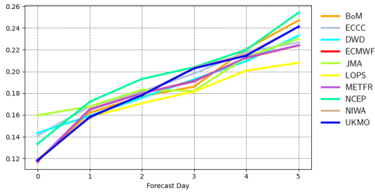
Scatter index | 10m wind speed | Gulf of Mexico 20231201 00z to 20240229 12z | waveapi lw wave prod mean_fair
