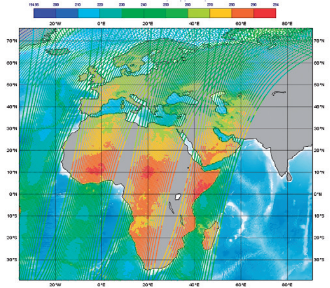
Figure 5 Brightness temperature values from the AMSU-A sensor onboard MetOp-A visualised in Metview 4. The values were extracted from the original BUFR file by Metview’s BufrPicker.
