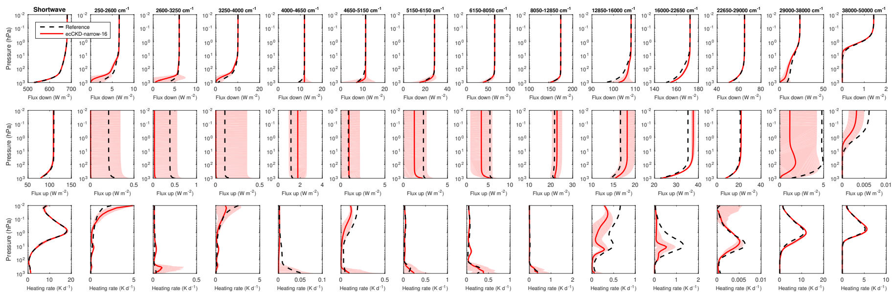
Evaluation of irradiances and heating rates for the broadband (leftmost column of panels) and the 13 narrow shortwave bands (other panels) of the global-nwp-narrow-16 CKD model. The black dashed and red solid lines correspond to the average of the 50 profiles for the “present-day” scenario, while the shaded regions encompass 95% of the error.
