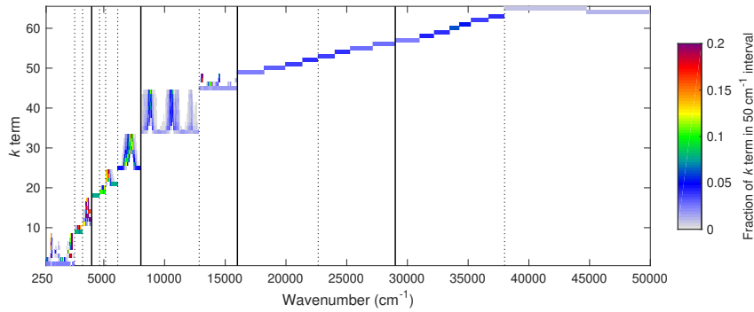
Illustration of the parts of the shortwave spectrum that contribute to each k term of the global-nwp-narrow-65 model.
