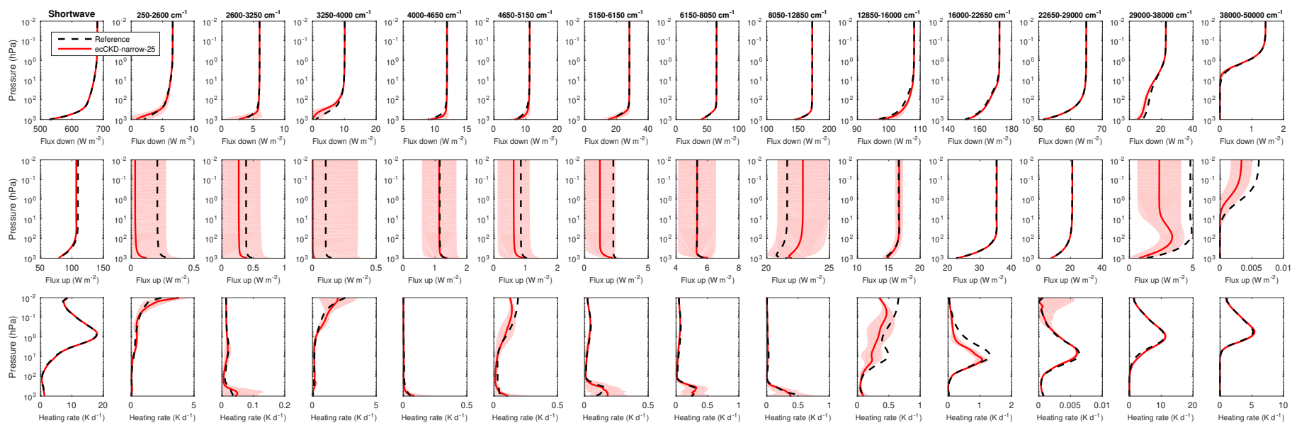
Evaluation of irradiances and heating rates for the broadband (leftmost column of panels) and the 13 narrow shortwave bands (other panels) of the global-nwp-narrow-25 CKD model. The black dashed and red solid lines correspond to the average of the 50 profiles for the “present-day” scenario, while the shaded regions encompass 95% of the error.
