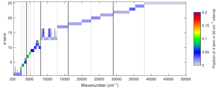
Illustration of the parts of the shortwave spectrum that contribute to each k term of the global-nwp-narrow-25 model.
