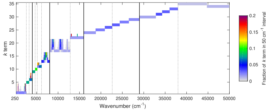
Illustration of the parts of the shortwave spectrum that contribute to each k term of the global-nwp-narrow-35 model.
