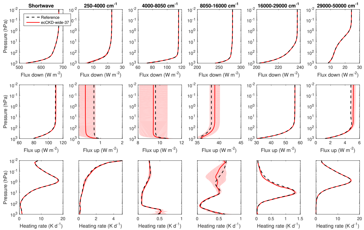
Evaluation of irradiances and heating rates for the broadband (leftmost column of panels) and the 5 wide shortwave bands (other panels) of the global-nwp-wide-37 CKD model. The black dashed and red solid lines correspond to the average of the 50 profiles for the “present-day” scenario, while the shaded regions encompass 95% of the error.
