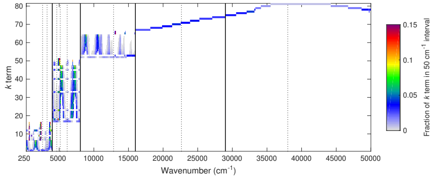
Illustration of the parts of the shortwave spectrum that contribute to each k term of the global-nwp-wide-81 model.
