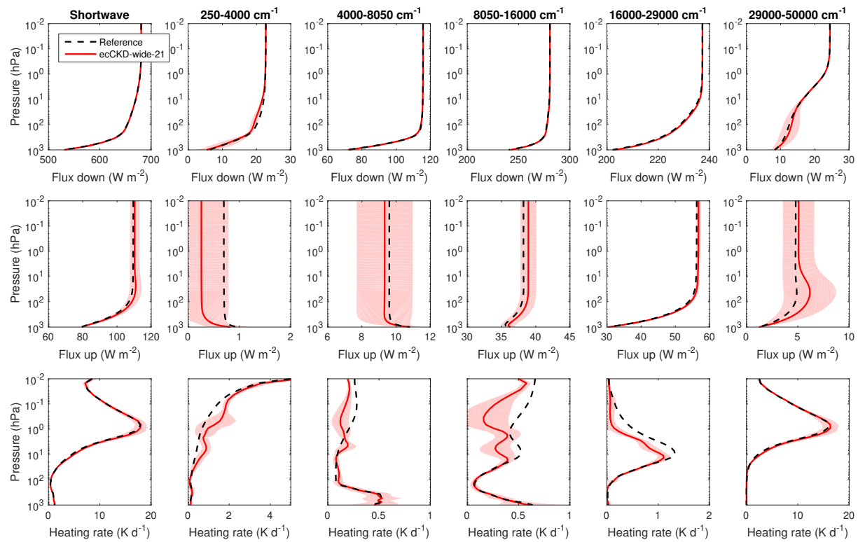
Evaluation of irradiances and heating rates for the broadband (leftmost column of panels) and the 5 wide shortwave bands (other panels) of the global-nwp-wide-21 CKD model. The black dashed and red solid lines correspond to the average of the 50 profiles for the “present-day” scenario, while the shaded regions encompass 95% of the error.
