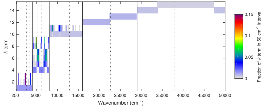
Illustration of the parts of the shortwave spectrum that contribute to each k term of the global-nwp-wide-15 model.
