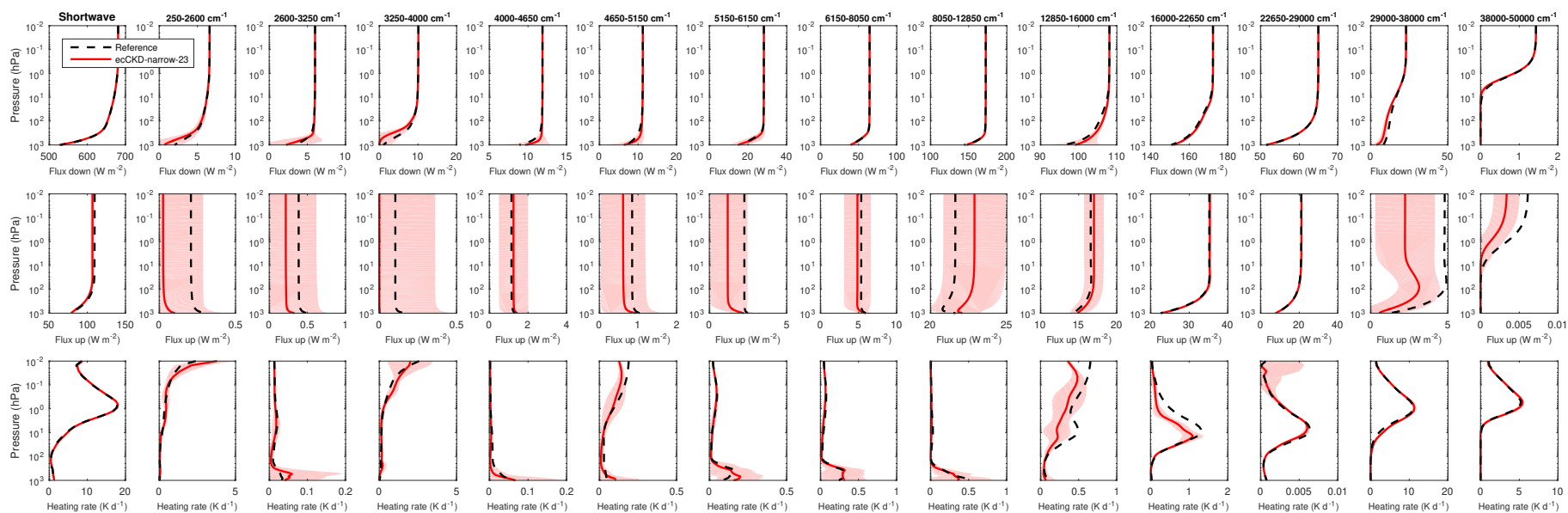
Evaluation of irradiances and heating rates for the broadband (leftmost column of panels) and the 13 narrow shortwave bands (other panels) of the global-nwp-narrow-23 CKD model. The black dashed and red solid lines correspond to the average of the 50 profiles for the “present-day” scenario, while the shaded regions encompass 95% of the error.
