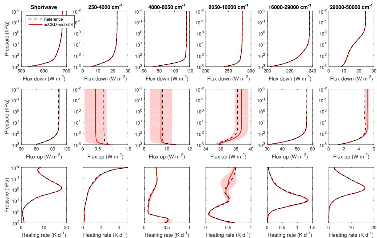
Evaluation of irradiances and heating rates for the broadband (leftmost column of panels) and the 5 wide shortwave bands (other panels) of the global-nwp-wide-58 CKD model. The black dashed and red solid lines correspond to the average of the 50 profiles for the “present-day” scenario, while the shaded regions encompass 95% of the error.
