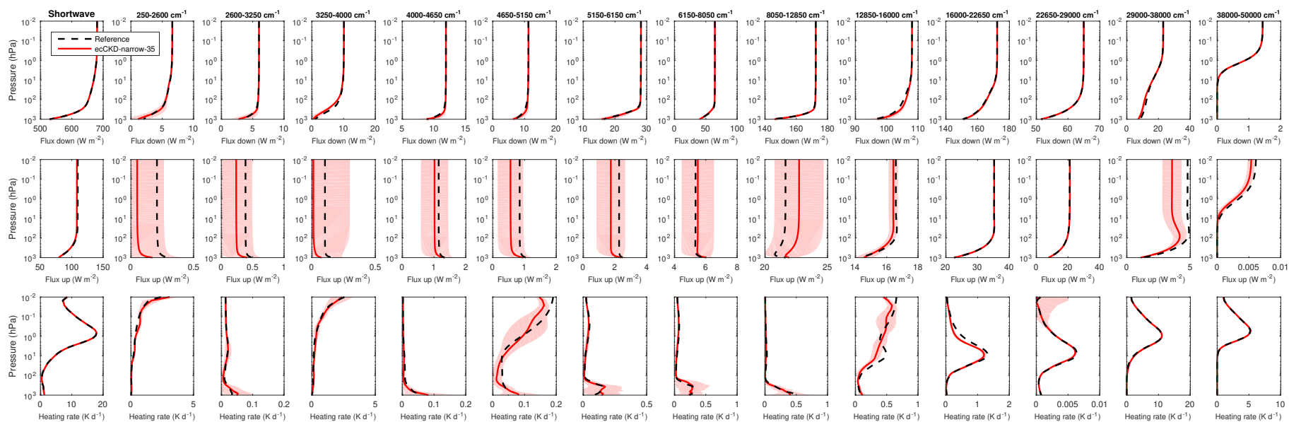
Evaluation of irradiances and heating rates for the broadband (leftmost column of panels) and the 13 narrow shortwave bands (other panels) of the global-nwp-narrow-35 CKD model. The black dashed and red solid lines correspond to the average of the 50 profiles for the “present-day” scenario, while the shaded regions encompass 95% of the error.
