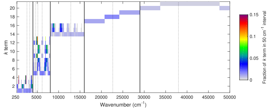
Illustration of the parts of the shortwave spectrum that contribute to each k term of the global-nwp-wide-21 model.
