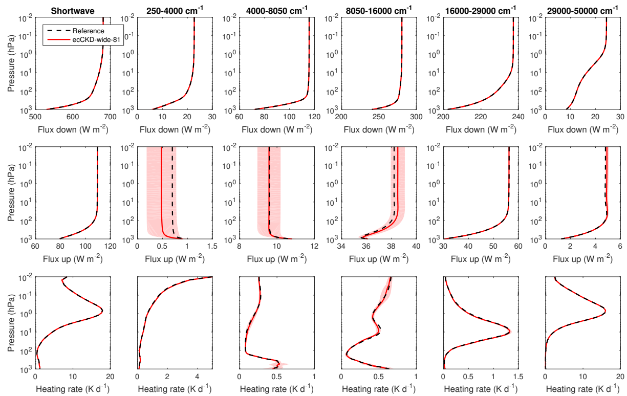
Evaluation of irradiances and heating rates for the broadband (leftmost column of panels) and the 5 wide shortwave bands (other panels) of the global-nwp-wide-81 CKD model. The black dashed and red solid lines correspond to the average of the 50 profiles for the “present-day” scenario, while the shaded regions encompass 95% of the error.
