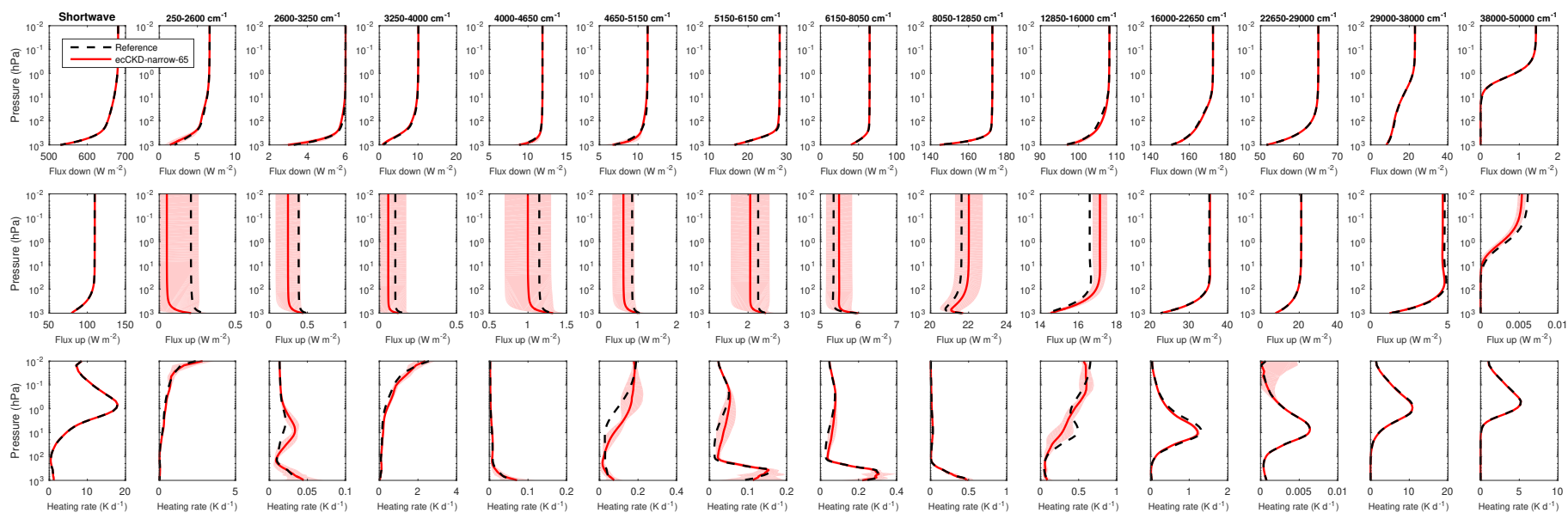
Evaluation of irradiances and heating rates for the broadband (leftmost column of panels) and the 13 narrow shortwave bands (other panels) of the global-nwp-narrow-65 CKD model. The black dashed and red solid lines correspond to the average of the 50 profiles for the “present-day” scenario, while the shaded regions encompass 95% of the error.
