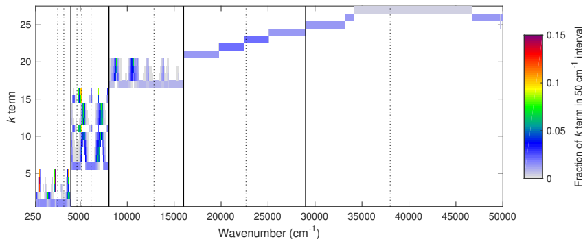
Illustration of the parts of the shortwave spectrum that contribute to each k term of the global-nwp-wide-27 model.
