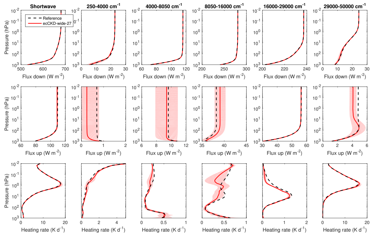
Evaluation of irradiances and heating rates for the broadband (leftmost column of panels) and the 5 wide shortwave bands (other panels) of the global-nwp-wide-27 CKD model. The black dashed and red solid lines correspond to the average of the 50 profiles for the “present-day” scenario, while the shaded regions encompass 95% of the error.
