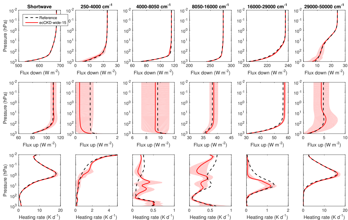
Evaluation of irradiances and heating rates for the broadband (leftmost column of panels) and the 5 wide shortwave bands (other panels) of the global-nwp-wide-15 CKD model. The black dashed and red solid lines correspond to the average of the 50 profiles for the “present-day” scenario, while the shaded regions encompass 95% of the error.
