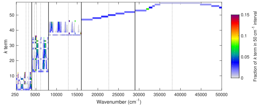
Illustration of the parts of the shortwave spectrum that contribute to each k term of the global-nwp-wide-58 model.
