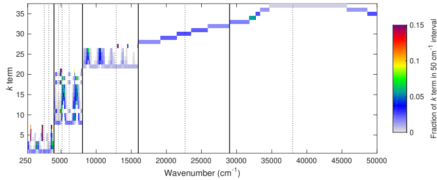
Illustration of the parts of the shortwave spectrum that contribute to each k term of the global-nwp-wide-37 model.
