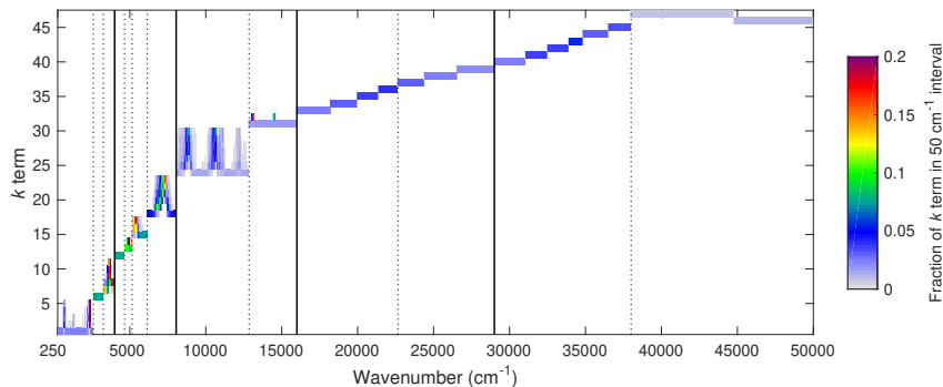
Illustration of the parts of the shortwave spectrum that contribute to each k term of the global-nwp-narrow-47 model.
