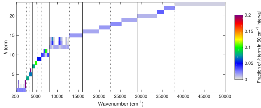
Illustration of the parts of the shortwave spectrum that contribute to each k term of the global-nwp-narrow-23 model.
