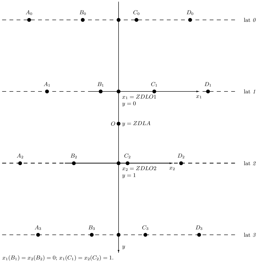
Figure 3.1: Interpolation horizontal grid for bilinear interpolations.
