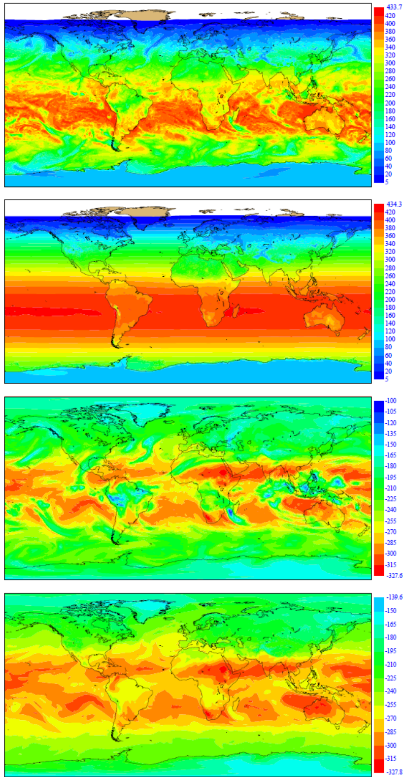
Figure 2: TSR, TSRC, TTR and TTRC averaged over the first 24 hours of the forecast started on 20120215 12 UTC ( W m^{-2} ).
