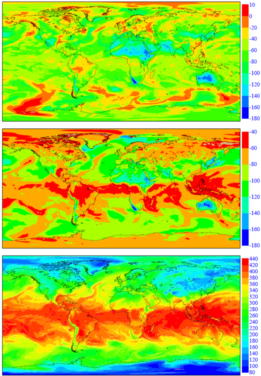
Figure 5: STR, STRC and STRD averaged over the first 24 hours of the forecast started on 20120215 12 UTC ( W m^{-2} ).
