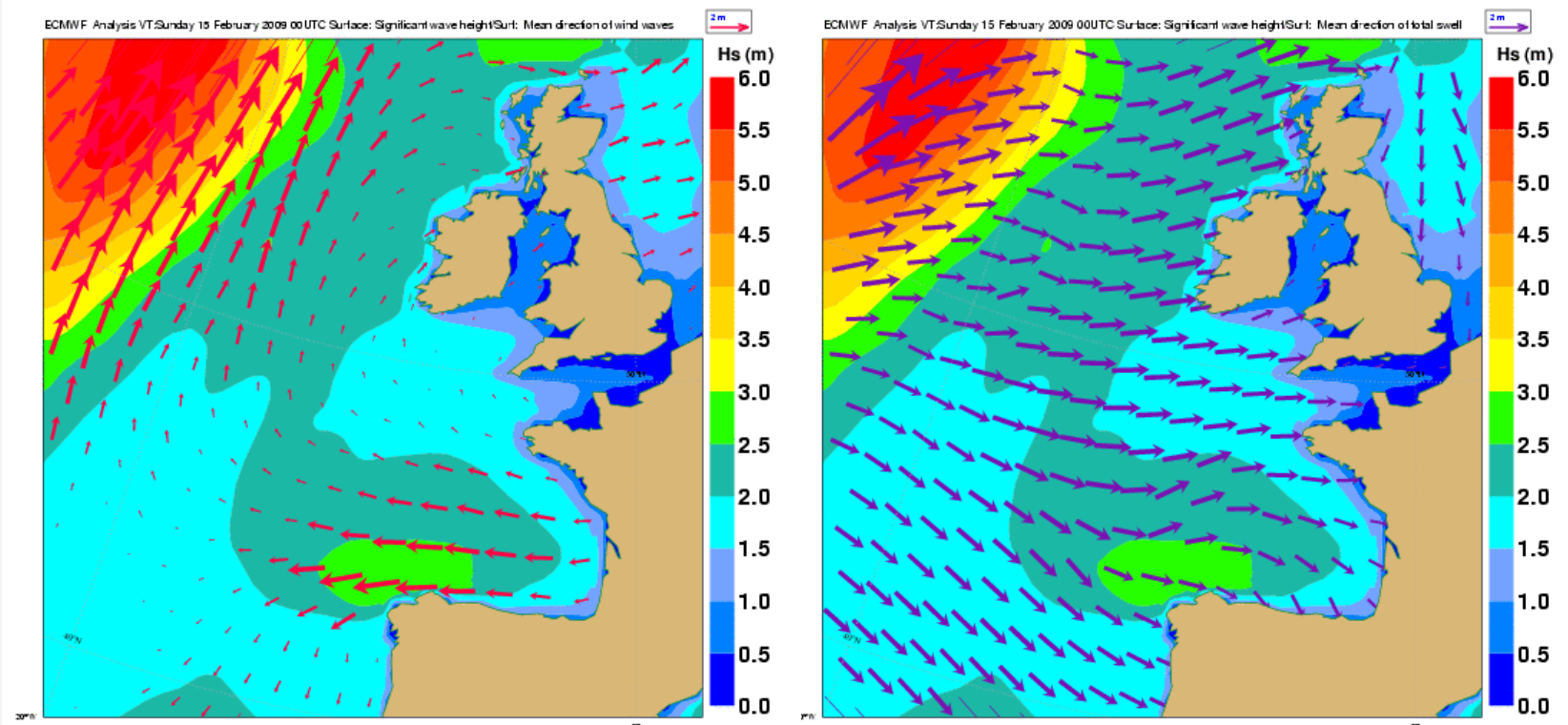
Wave height and windsea mean direction: Analysis : 15 February 2009, 00 UTC
