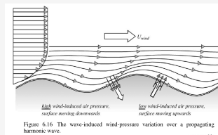
Figure 6.16 The wave-induced wind-pressure variation over a propagating harmonic wave.
